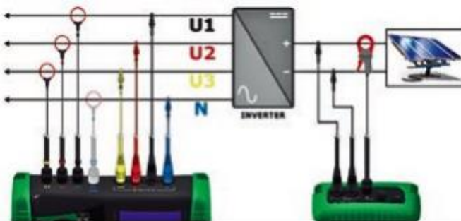
Connection diagram in a photovoltaic network
